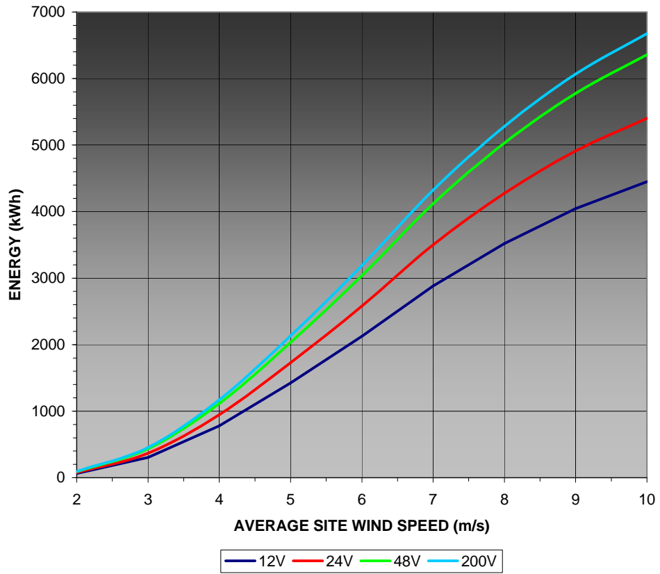
ANNUAL ENERGY kWh 10min BINS - COASTAL
